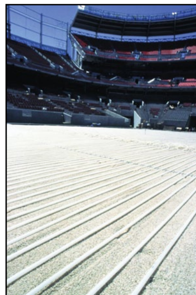
Figure 11.6 – Turf Conditioning in a Stadium
