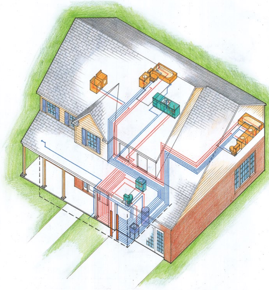
Figure 6.2 – PEX Pipes in a Parallel Design
