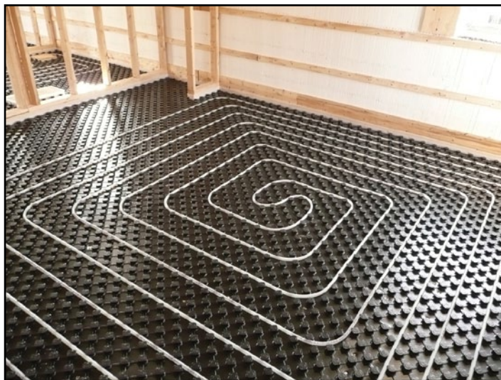
Figure 11.1 – Radiant Floor Heating Piping in a Residential Application
