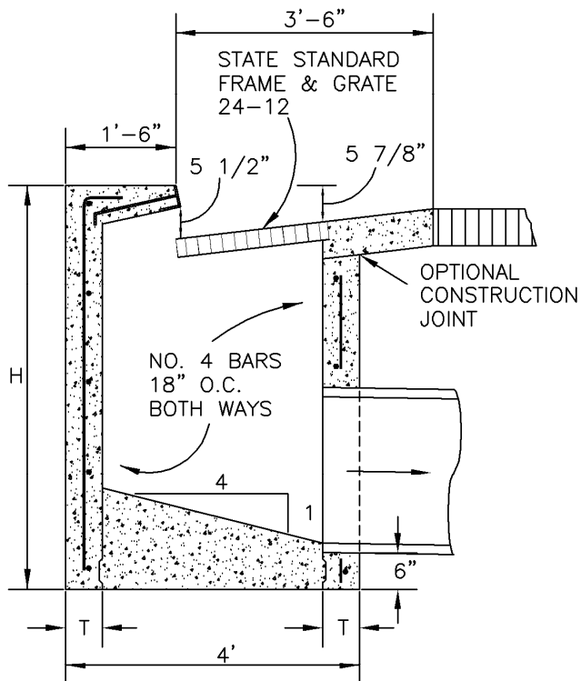
SECTION
