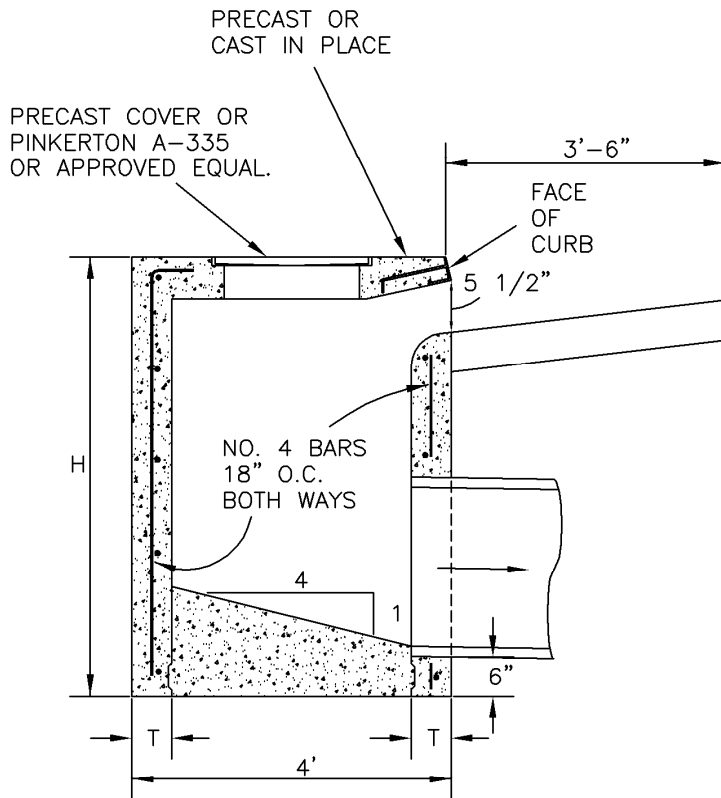
SECTION
