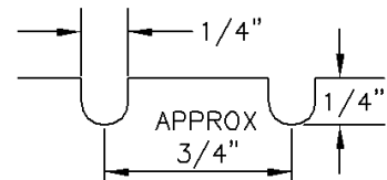
GROOVE DETAIL
