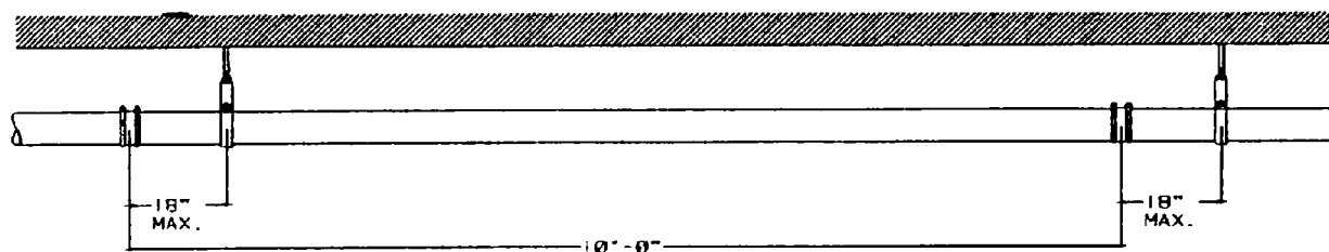
Figure 7—Hanger Spacing for Aboveground Installation.
