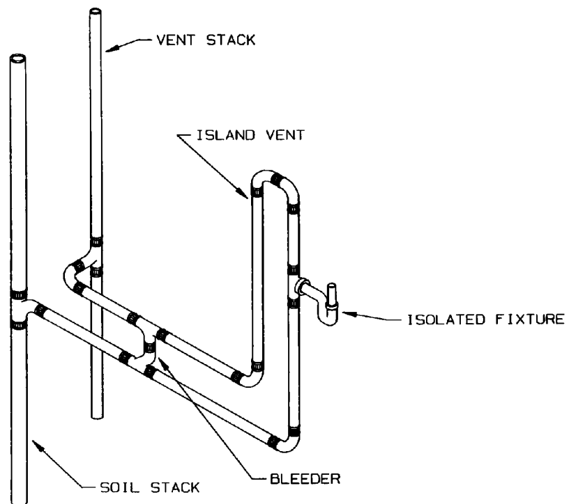
Figure 12—Island Vent.
