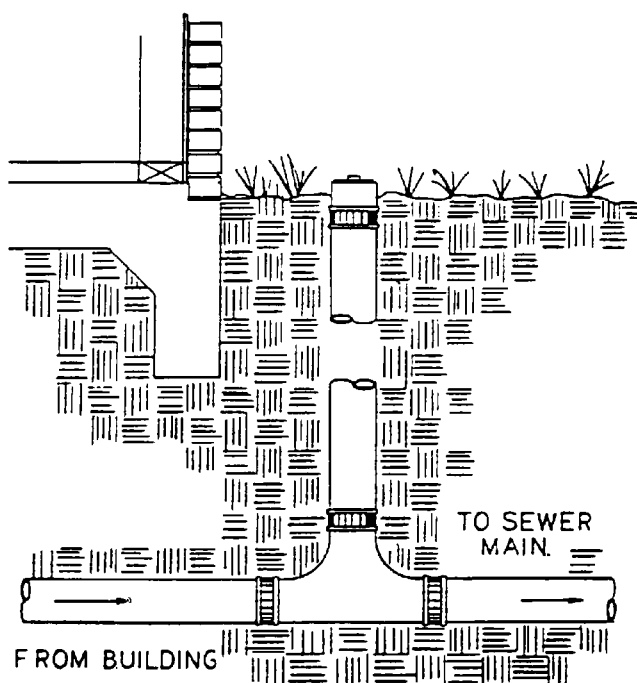
Figure 20—Twin Cleanout.
