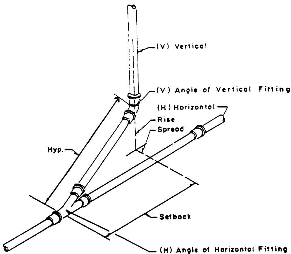
Figure 5—Explanation of the Compound Offset Table.
