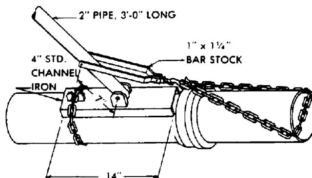
Figure 4—Pulling Assembly.
