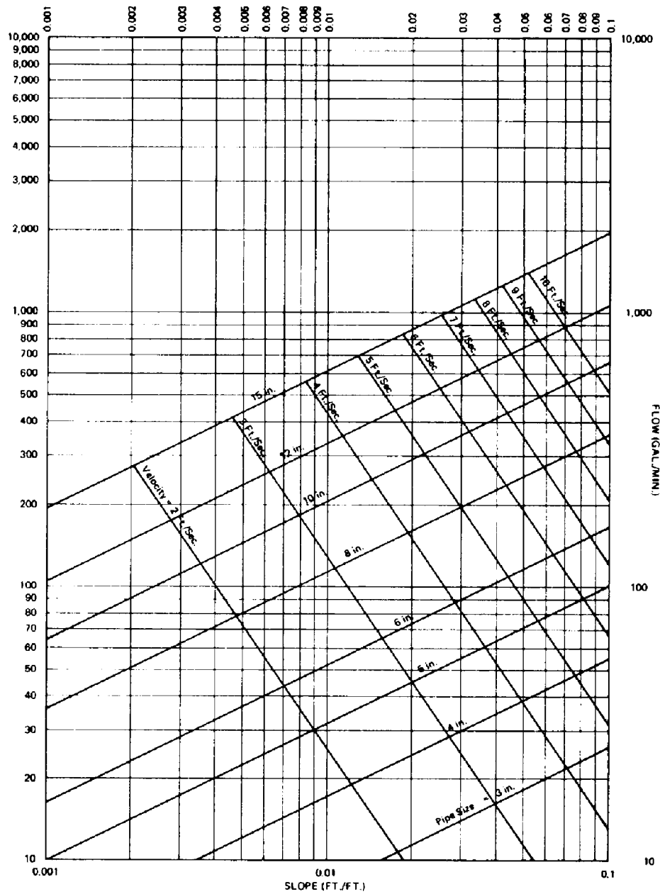
Figure 3—Velocity and Flow in Cast Iron Soil Pipe, Sewers, and Drains (Based on Manning's Formula, With n=0.012 ).
