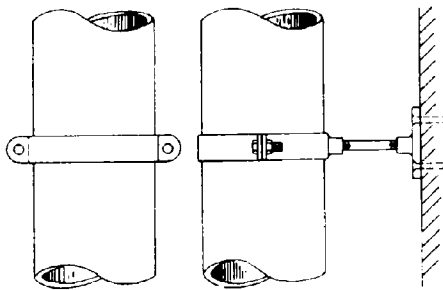
Figure 14—One Hole Strap for Vertical Pipe.
