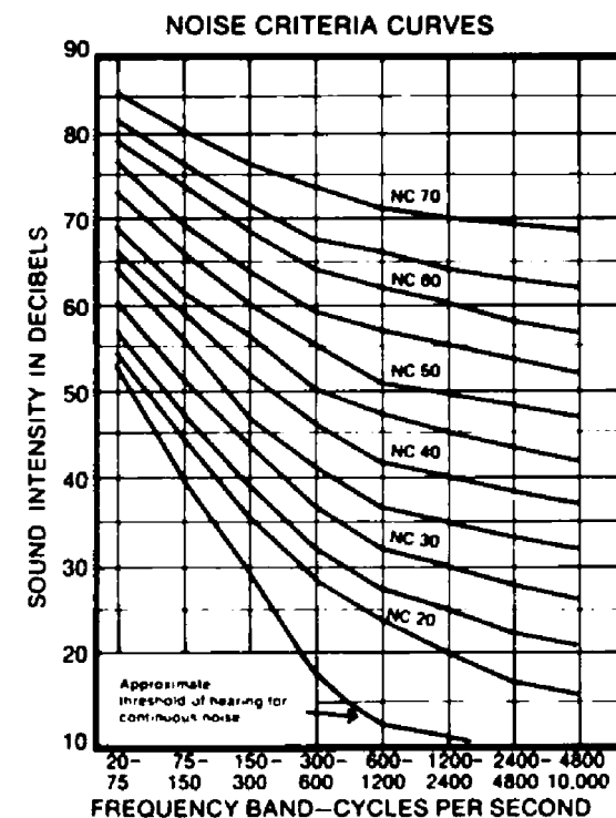
Figure 1—Recommended Noise Criteria for Rooms.
