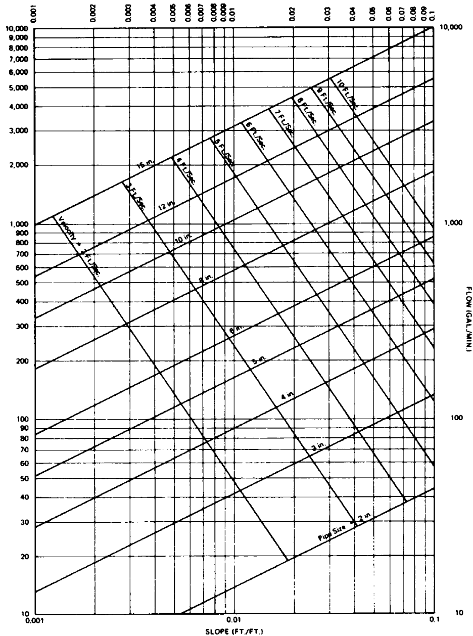
Figure 6—Velocity and Flow in Cast Iron Soil Pipe, Sewers, and Drains (Based on Manning's Formula, With n=0.012 ).
