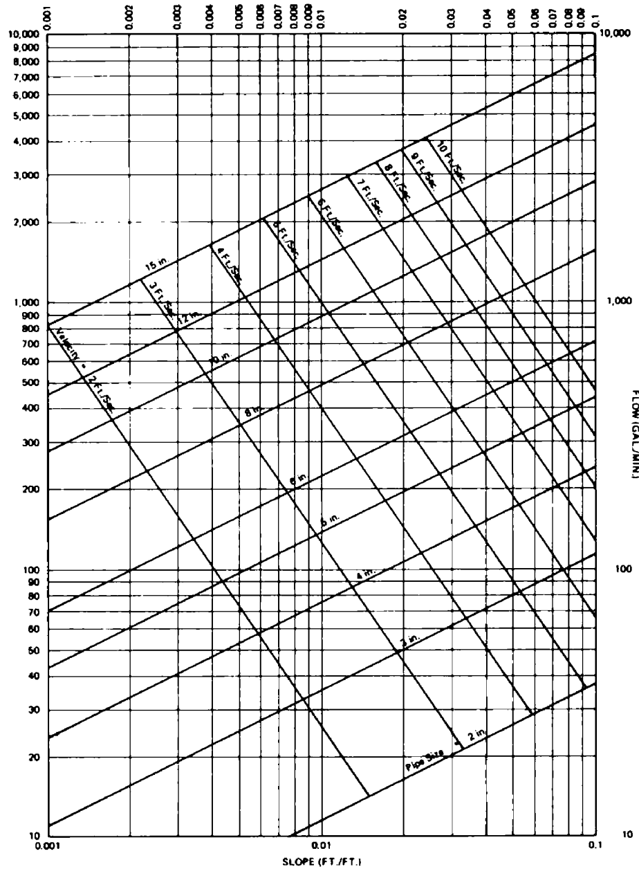
Figure 5—Velocity and Flow in Cast Iron Soil Pipe, Sewers, and Drains (Based on Manning's Formula, With n=0.012 ).
