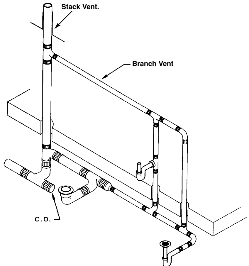
Figure 8—Branch Vent.
