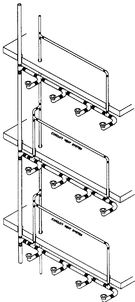
Figure 9—Circuit Venting.
