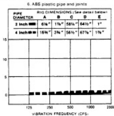
Figure 5—Vibration Drops Across the Pipe Joints of Six DWV Systems.
