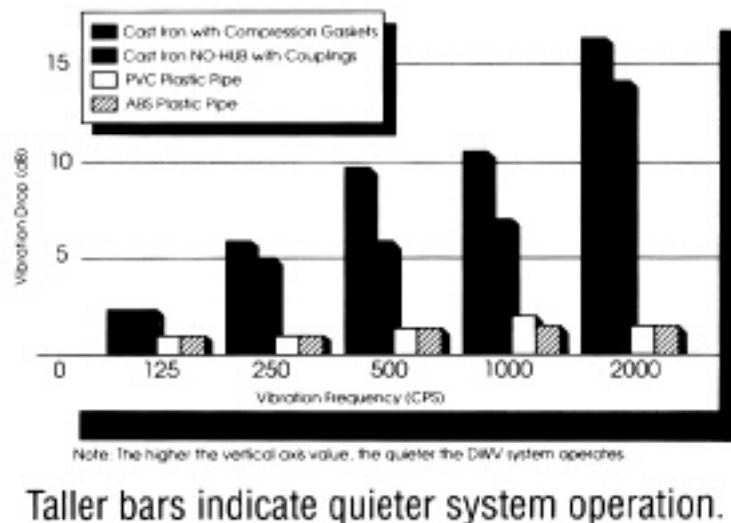
Figure 2—Noise Muffling Qualities of DWV Materials.
