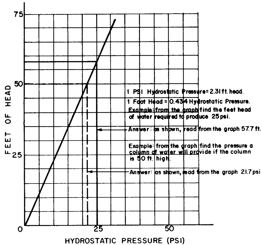
Figure 2 Hydrostatic Conversion Graph. Feet of Head Into Pounds Per Sq. In.
