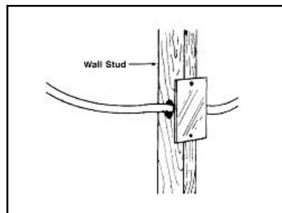
Nail plate
