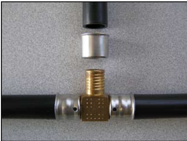
Figure 5.9 – Metal Insert Fitting with Stainless Steel Press Sleeve
