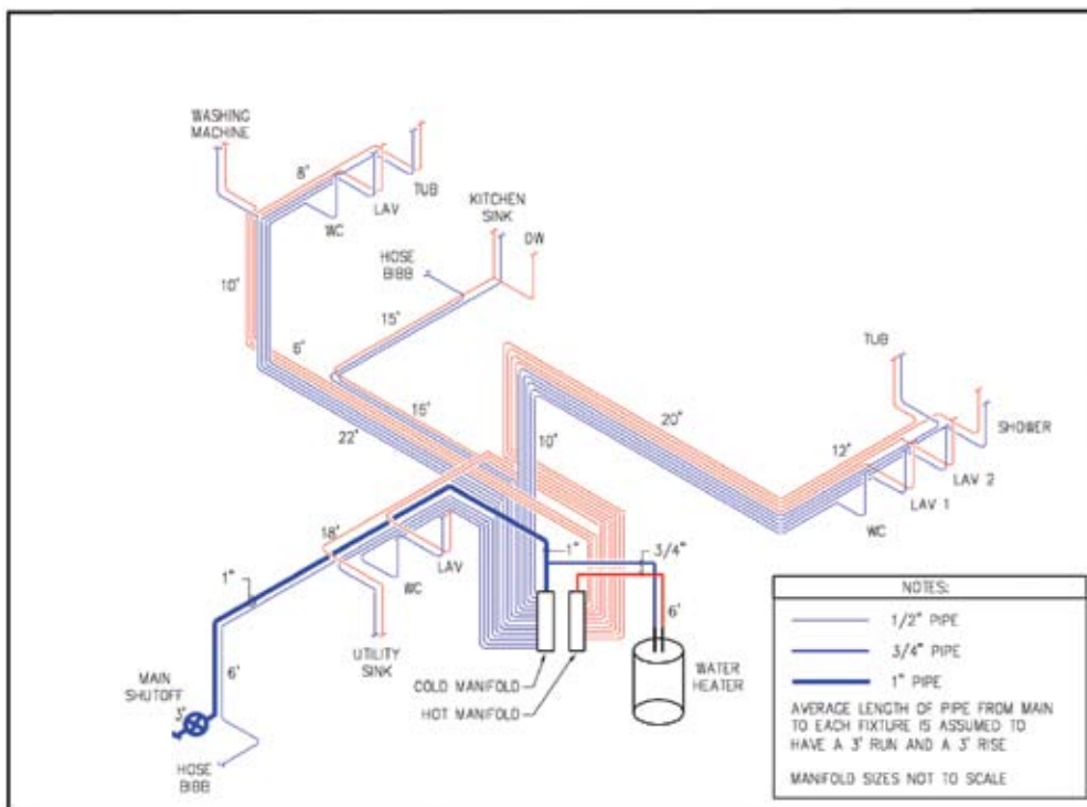
Figure 7.2 – Home-Run Isometric Riser for the Colonial House
